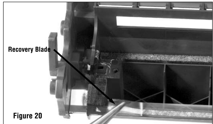
Use a pair of needle nose pliers to remove the Recovery Blade.
