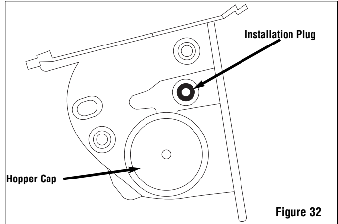
Install the Contact Side End Plate.
