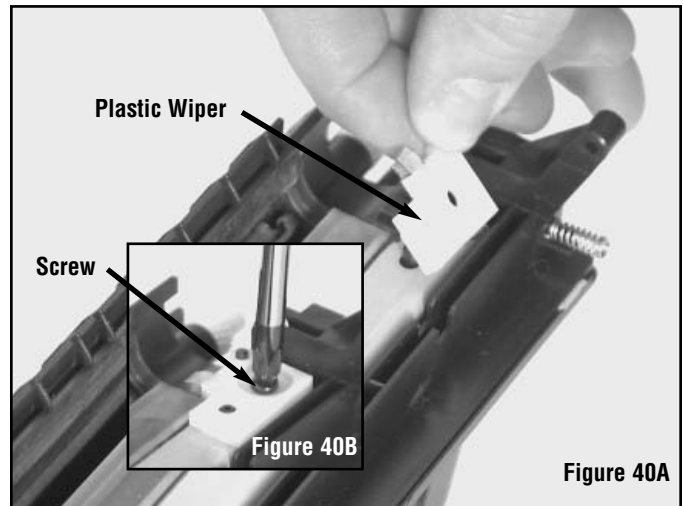
Install the Plastic Wipers.
