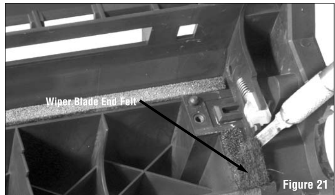
Using a scraper tool remove the Wiper Blade End Felts.
