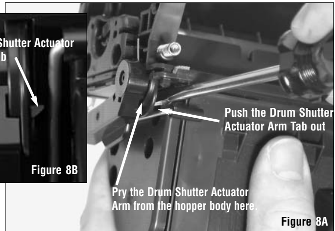
Remove the Drum Shutter Actuator Arm from the hopper body using a screw driver.
