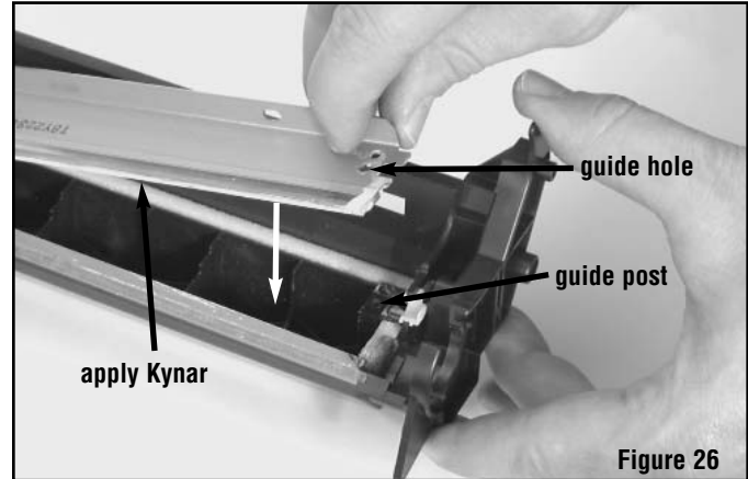
Figure 26 Apply Kynar lubricating powder to the working edge; then, line up the guide hole with guide post and install the Wiper Blade.
