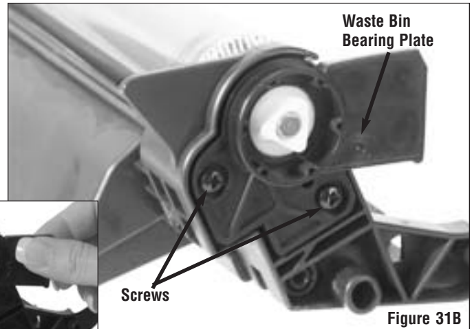
Figure 31B Install the Waste Bin Bearing Plate securing it with 2 screws.
