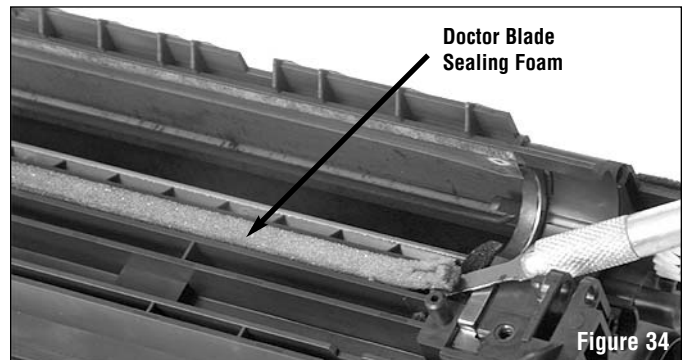
Using a scraper tool remove the Doctor Blade Sealing Foam.
