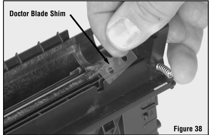
Install the Doctor Blade Shims if necessary.
