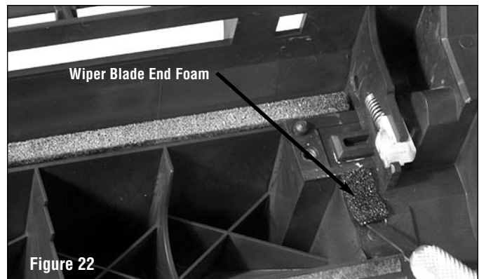
Use the scraper tool to remove the Wiper Blade End Foams.
