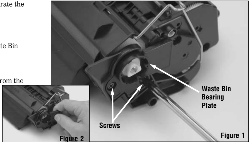
Remove the Waste Bin Bearing Plate by removing the 2 screws.
