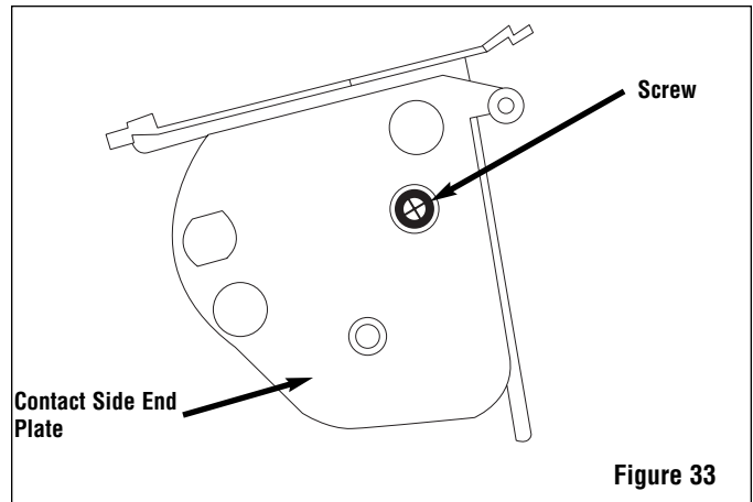
Secure the Contact Side End Plate using the screw provided.
