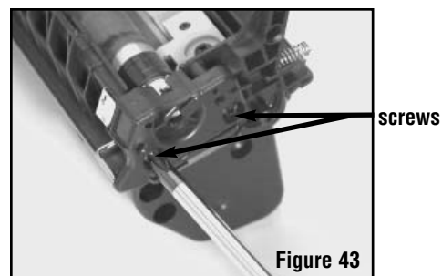
Install the screws securing the end plate to the hopper body.
