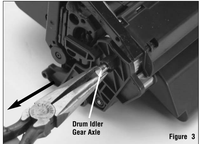
Remove the Drum Idler Gear Axle with needle nose pliers.
