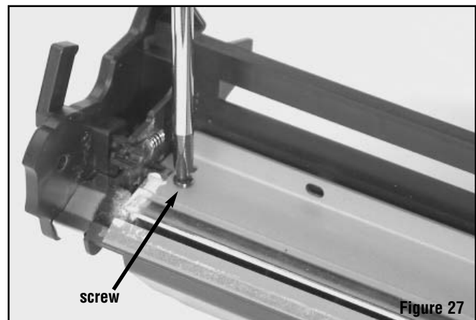
Figure 27 Secure the Wiper Blade with 2 screws one on each end.
