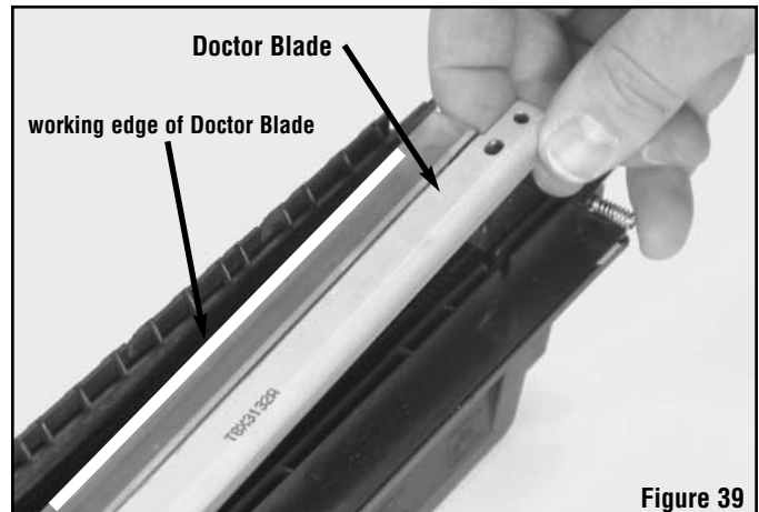
Install the Doctor Blade in the hopper body.
